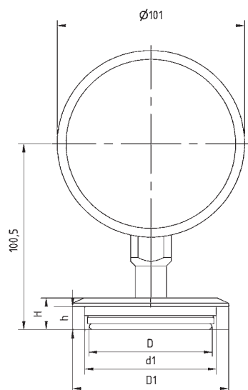
Pressure gauge NG 100 with MD 63
