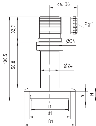
Pressure transducer DMU 02 Vario VT
