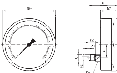
Centre back connection (NG 160 only)
