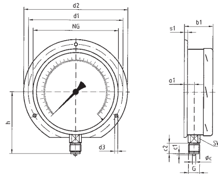
Bottom connection, back flange (NG 160 only)
