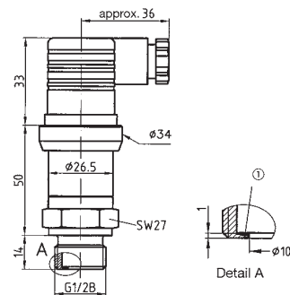
DMU 01 VM with connection G \frac{1}{2} B DIN 3852 type E with flush diaphragm DMU 01 VM
