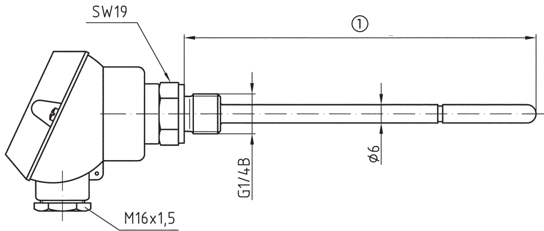
Type WTh 23
