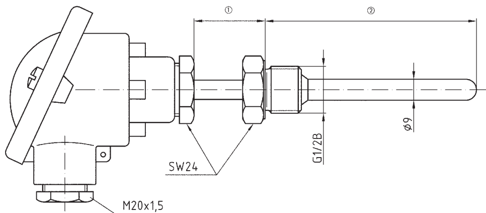
Type WTh 24
